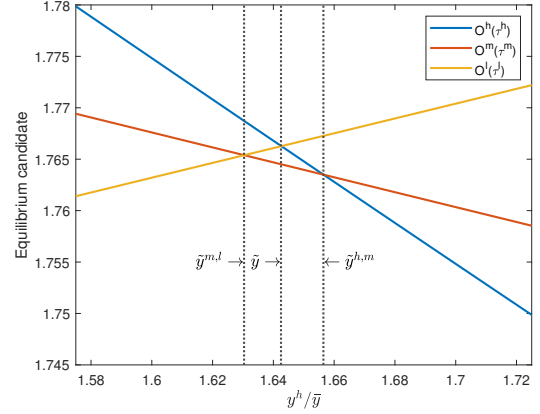
(b) Balanced: \pi^r(v) = 49/100 , \pi^p(v) = 1/2
